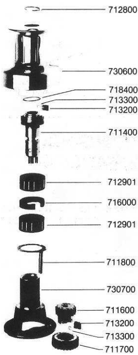
No. 28 Two Speed Winch
