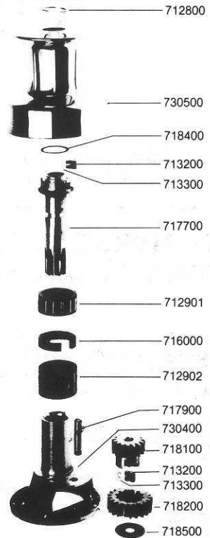
No. 46 Two Speed Winch
