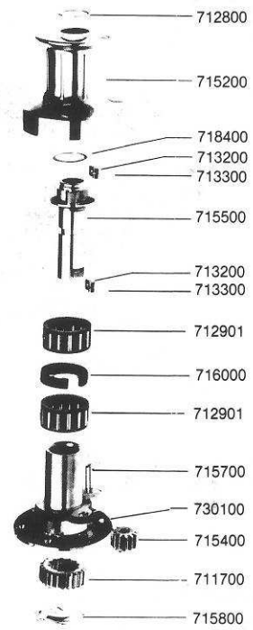
No. 16 Two Speed Winch
