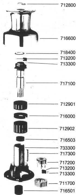
No. 40 Two Speed Winch
