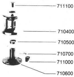
No. 6 Single Speed Winch
